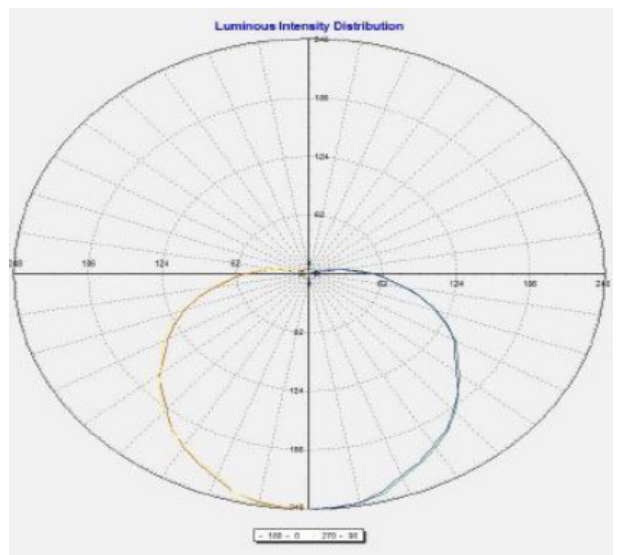
TECHNO CANOPY 180
