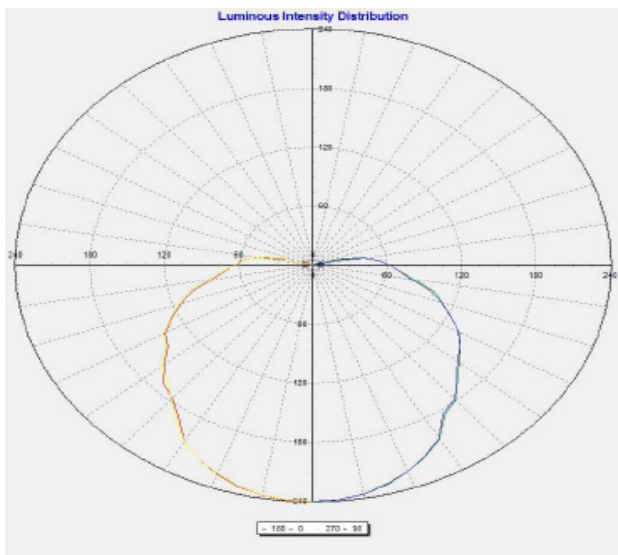
TECHNO CANOPY 130
