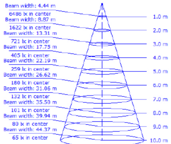
TECHNO CANOPY 180
